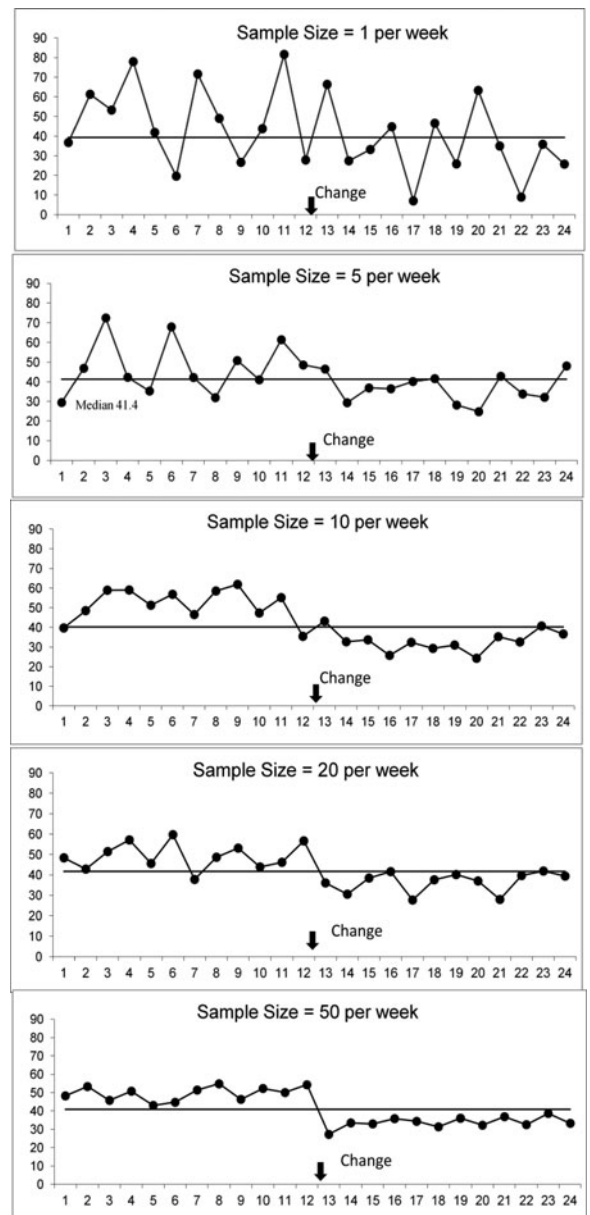
Figure 1. Sample size on a run chart and ability to detect change.
